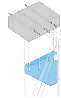
Sistema DECK INTEGRATED SUPPORT
